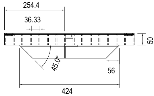
GRATE SECTION DETAIL
