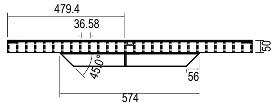
GRATE SECTION DETAIL
