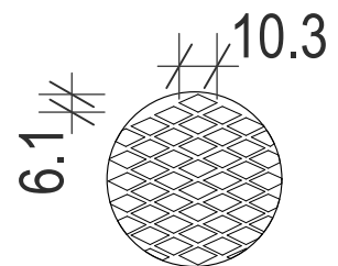
RH3030 MESH DETAIL
