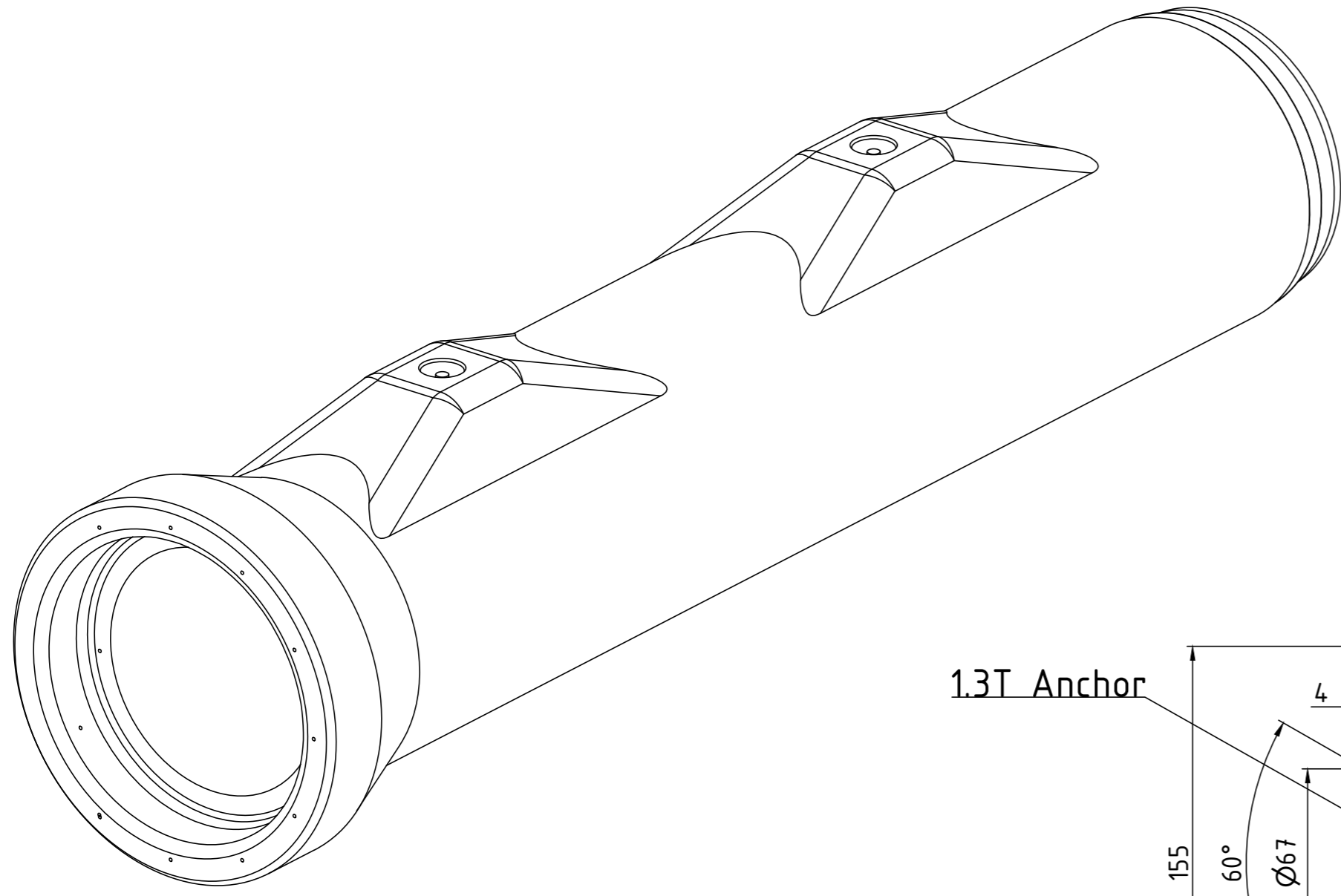
3D View
