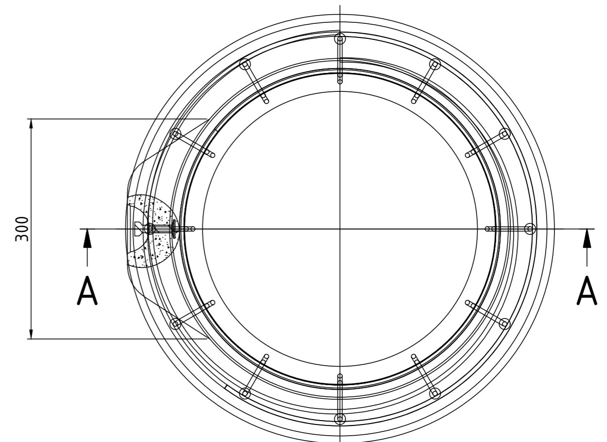
Plan View
