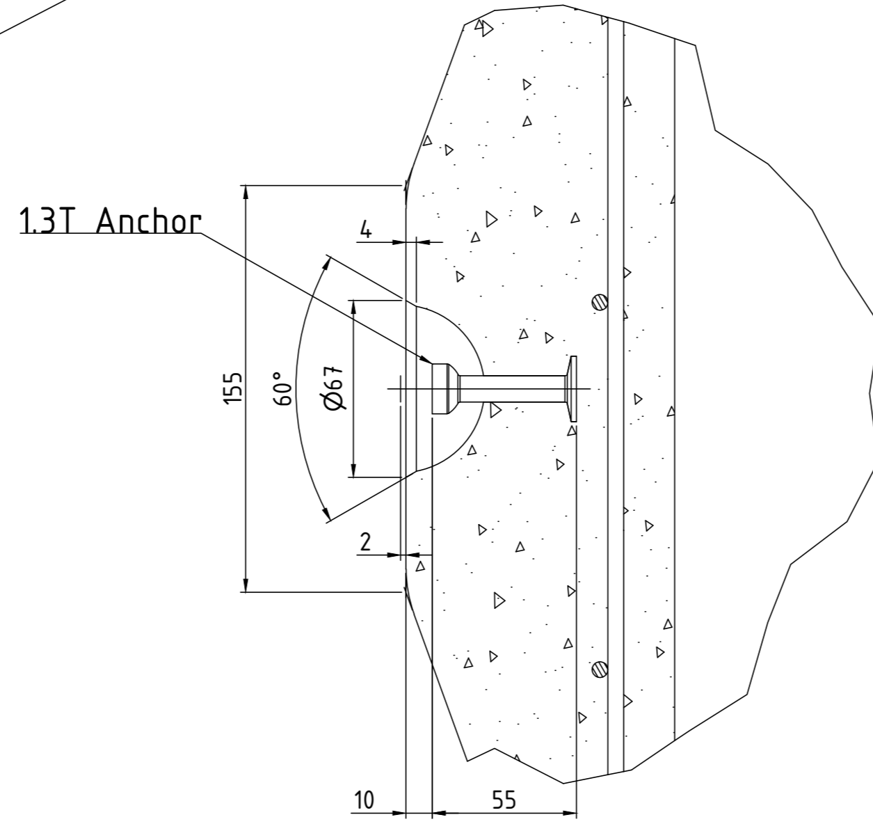
Detail B
