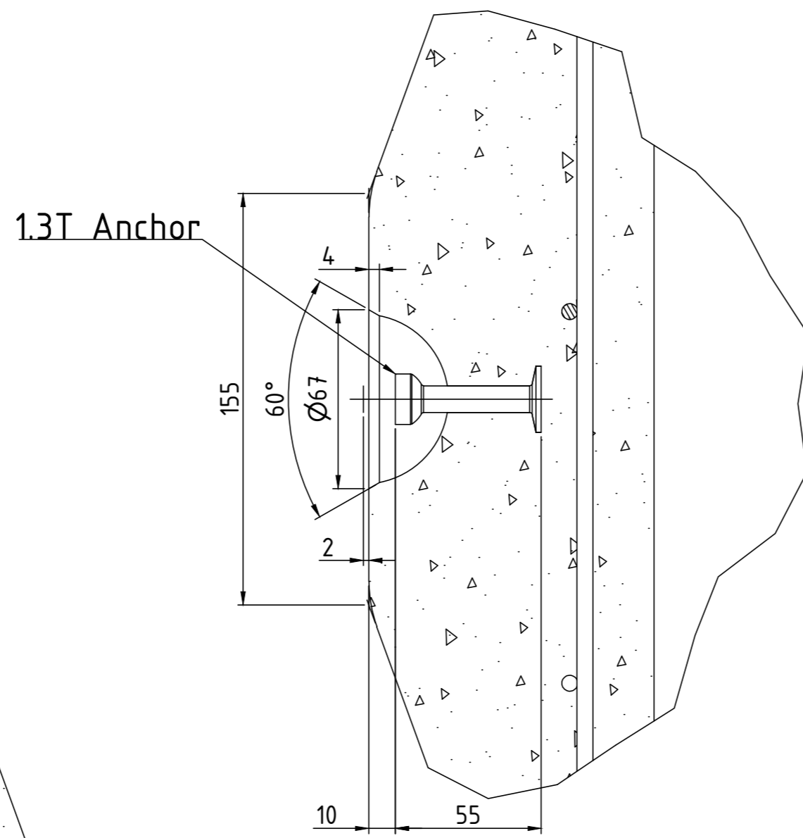
Detail B
