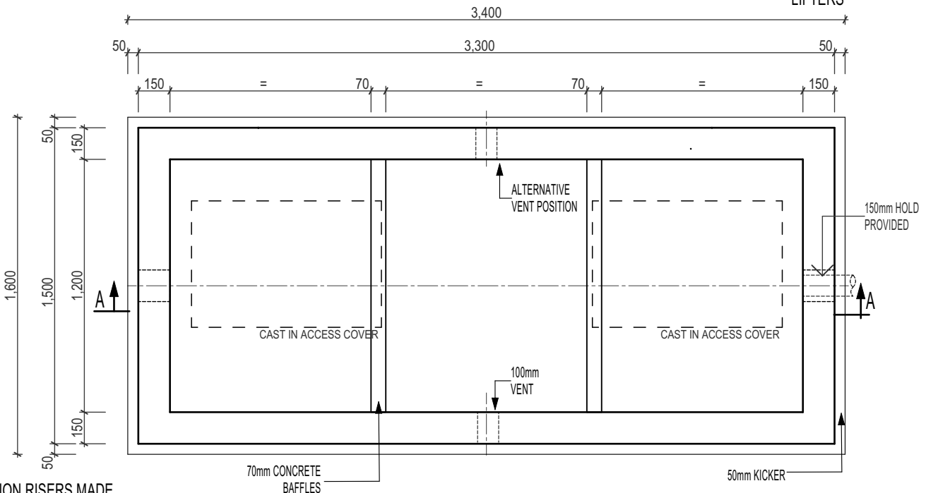
PLAN
