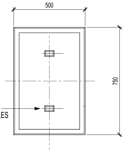
PLAN - INSERT
